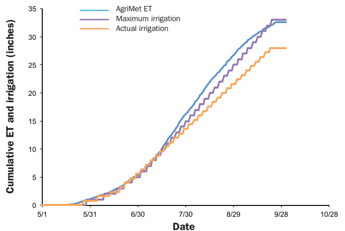
Figure 3. AgriMet-estimated cumulative corn ET, Bliss, ID, 2005, and the actual cumulative irrigation applied. The maximum irrigation curve represents net center pivot irrigation system capacity at 7 gpm/acre and 85% application efficiency.
