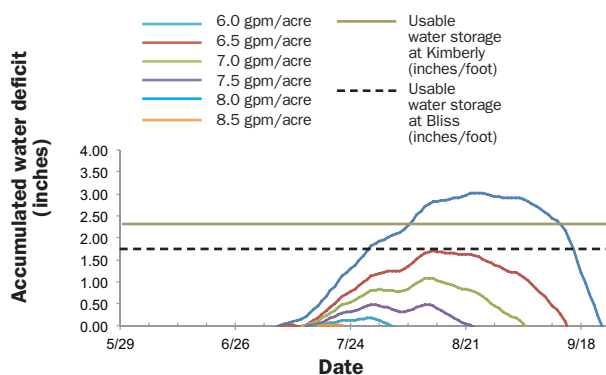
Figure 9. Accumulated water deficit (AgriMet ET – water applied) with center pivot capacities of 6–8.5 gpm/acre, Kimberly, ID, 2006.
