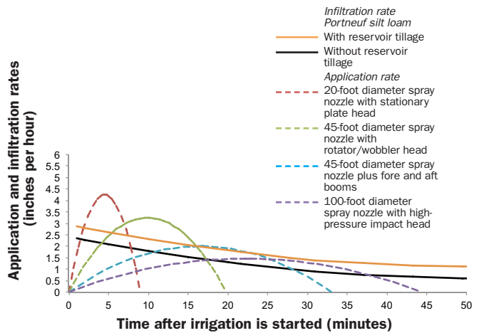
Figure 15. Estimated water application rates from three sprinkler devices under the last (outer) pivot span and from the 45-foot-wetted-diameter device with alternate fore-aft booms as compared with the infiltration rates with and without reservoir tillage for a Portneuf silt loam soil.
