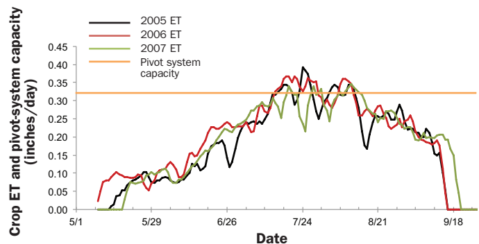
Figure 6. AgriMet-estimated crop water use and pivot system capacity for corn at Kimberly, ID. ET data are plotted as a 3-day moving average to smooth daily fluctuations.
