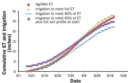
Figure 4. Irrigation system performance relative to AgriMet-estimated, 30-year average corn ET, Kimberly, ID. Assumed center pivot capacity is 0.28 inch/day with net irrigation of 6.5 gpm/acre at 80% application efficiency.
