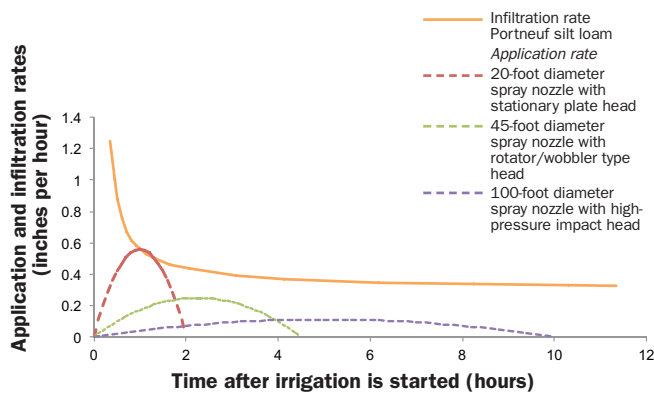
Figure 11. Estimated water application rates from three sprinkler devices under the first pivot span as compared with the infiltration rate for a Portneuf silt loam soil, Kimberly, ID.
