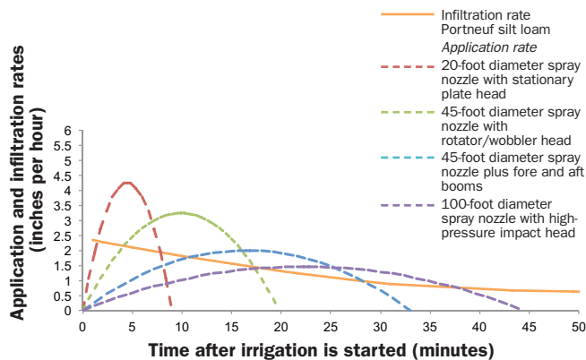
Figure 12. Estimated water application rates from three sprinkler devices under the last (outer) pivot span and from the 45-foot-wetted-diameter device with alternate fore-aft booms as compared with the infiltration rate for a Portneuf silt loam soil, Kimberly, ID.
