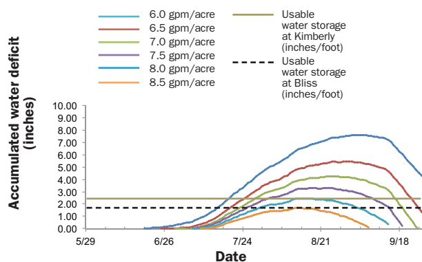
Figure 8. Accumulated water deficit (AgriMet ET – water applied) with center pivot capacities of 6–8.5 gpm/acre, Bliss, ID, 2006.
