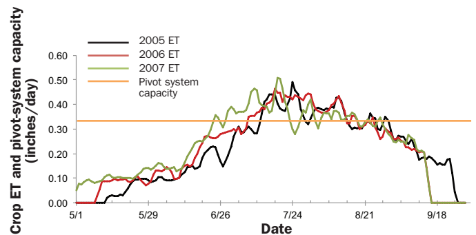
Figure 7. AgriMet-estimated crop water use and pivot system capacity for corn at Bliss, ID. ET data are plotted as a 3-day moving average to smooth daily fluctuations.
