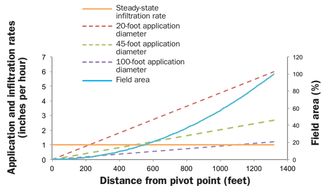
Figure 16. Steady-state infiltration rate on a sandy loam soil, sprinkler application rate, and percentage of field area with distance from pivot point.
