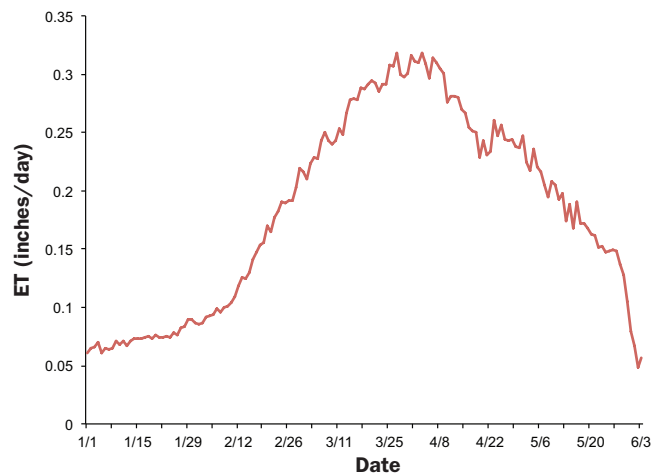
Figure 2. Average 30-year ET requirements for corn in the Magic Valley, estimated by AgriMet.
