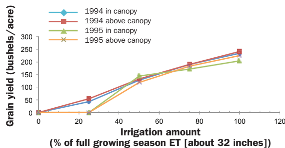
Figure 5. Grain yield response to irrigation treatment, Bushland, TX, 1994 and 1995. (Source: Schneider, A. D., and T. A. Howell. 1998. LEPA and spray irrigation of corn—Southern High Plains. Trans. ASAE 41(5):1391–1396.)
